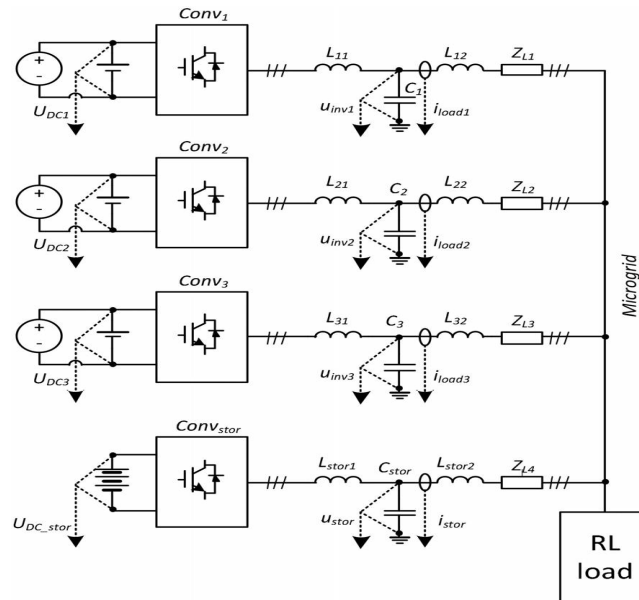
Fig. 7: Block scheme of simulation model.
