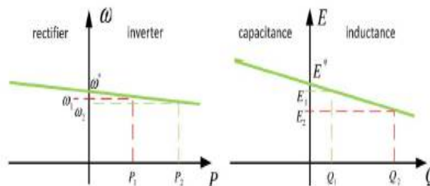
Fig. 2: P- \omega and Q-E droop characteristics.
